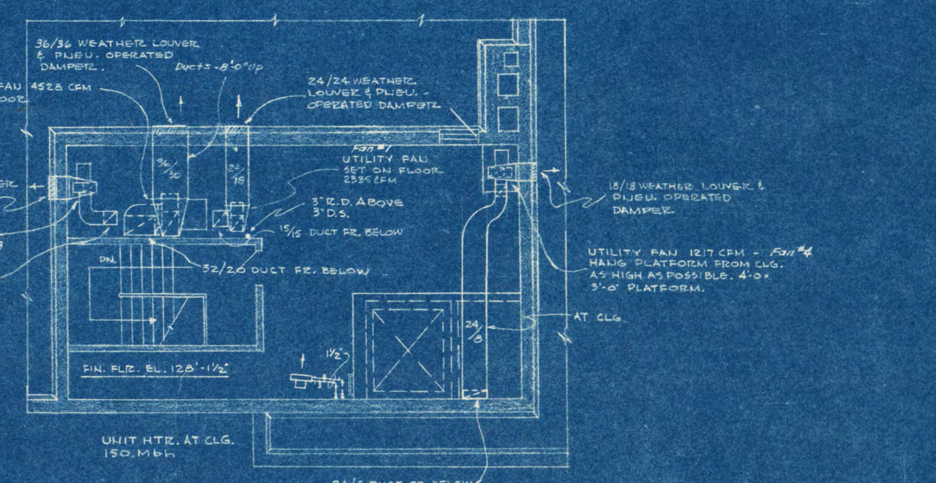
PENTHOUSE FLOOR PLAN SCALE 1/8" = 1'-0"
