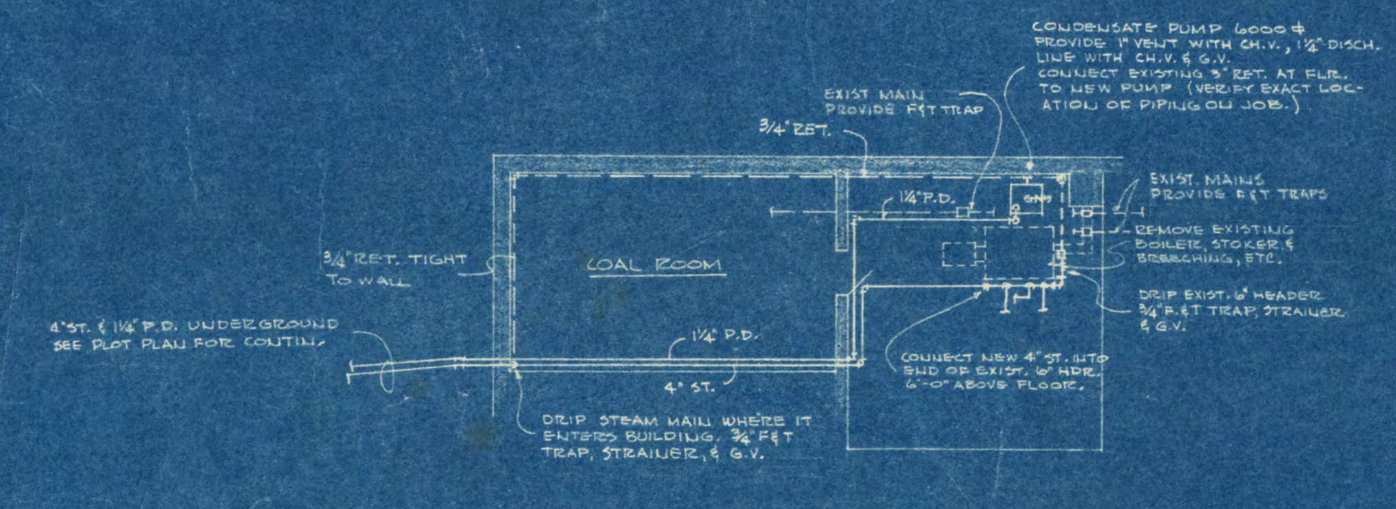
LAYOUT OF COAL & BOILER ROOMS IN WHITNEY RESIDENCE SCALE 1/8" = 1'-0" VERIFY ALL LOCATIONS ON JOB
