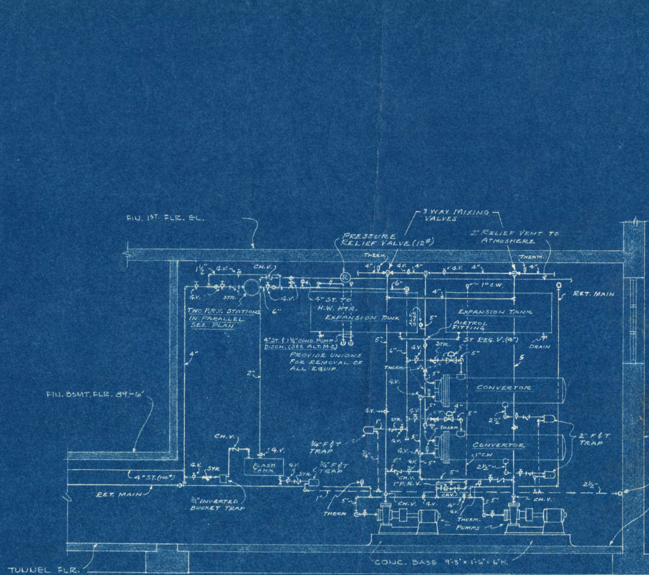
CONVERTER PIPING DETAIL SCALE: 3/8" = 1'-0"
