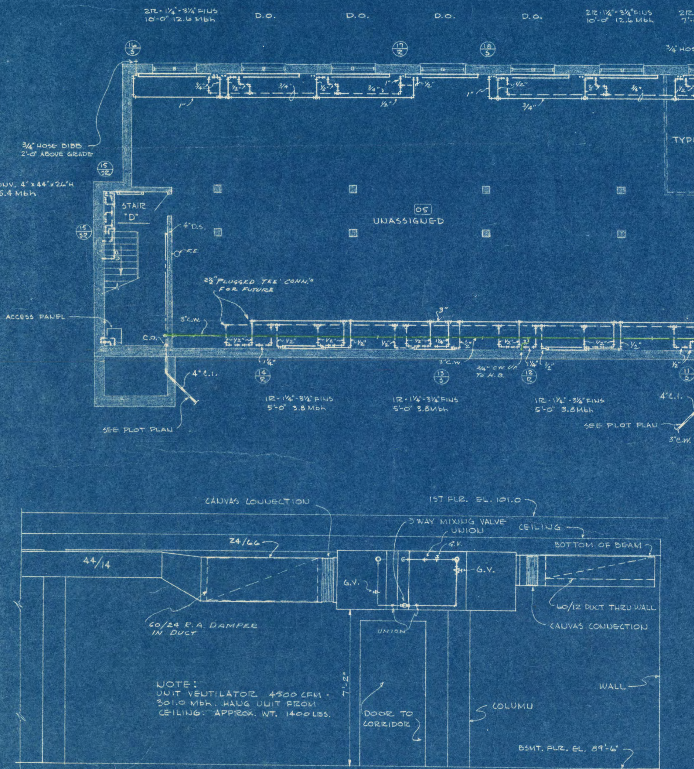
DETAIL OF UNIT VENTILATOR FOR TELEVISION & ACTIVITIES ROOMS SCALE: 3/8" = 1'-0"
