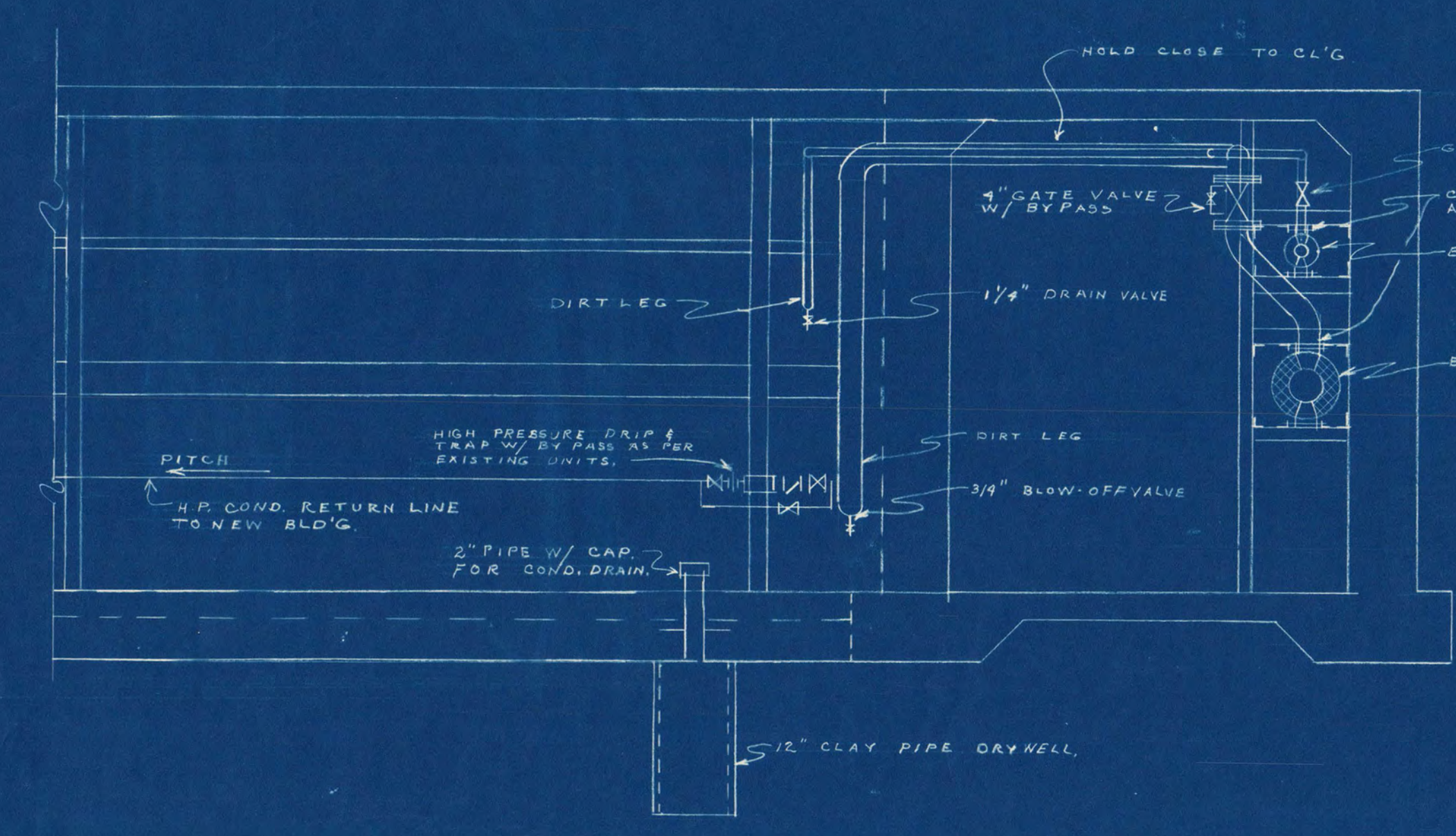
TUNNEL PIPING TAKE-OFFS SECTION 3 SCALE 1/2" = 1'-0"
