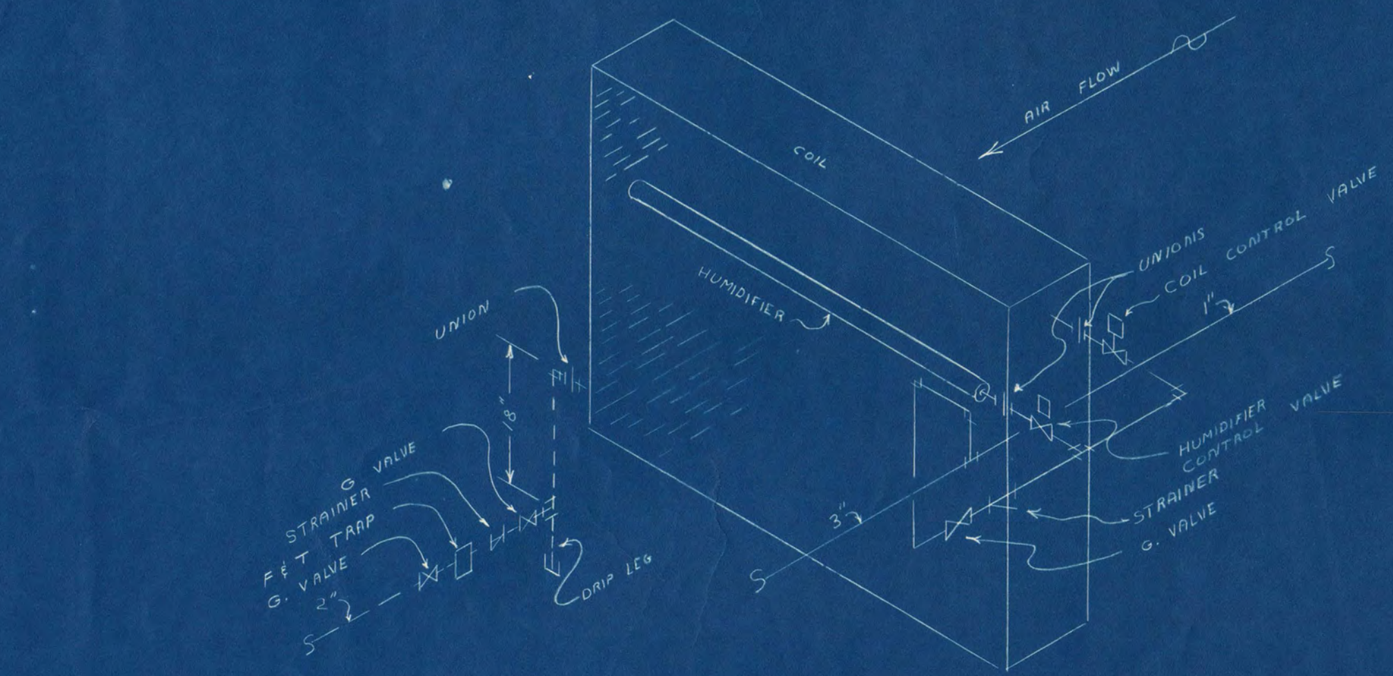
PENTHOUSE H.V. UNIT COIL PIPING DETAIL NO SCALE
