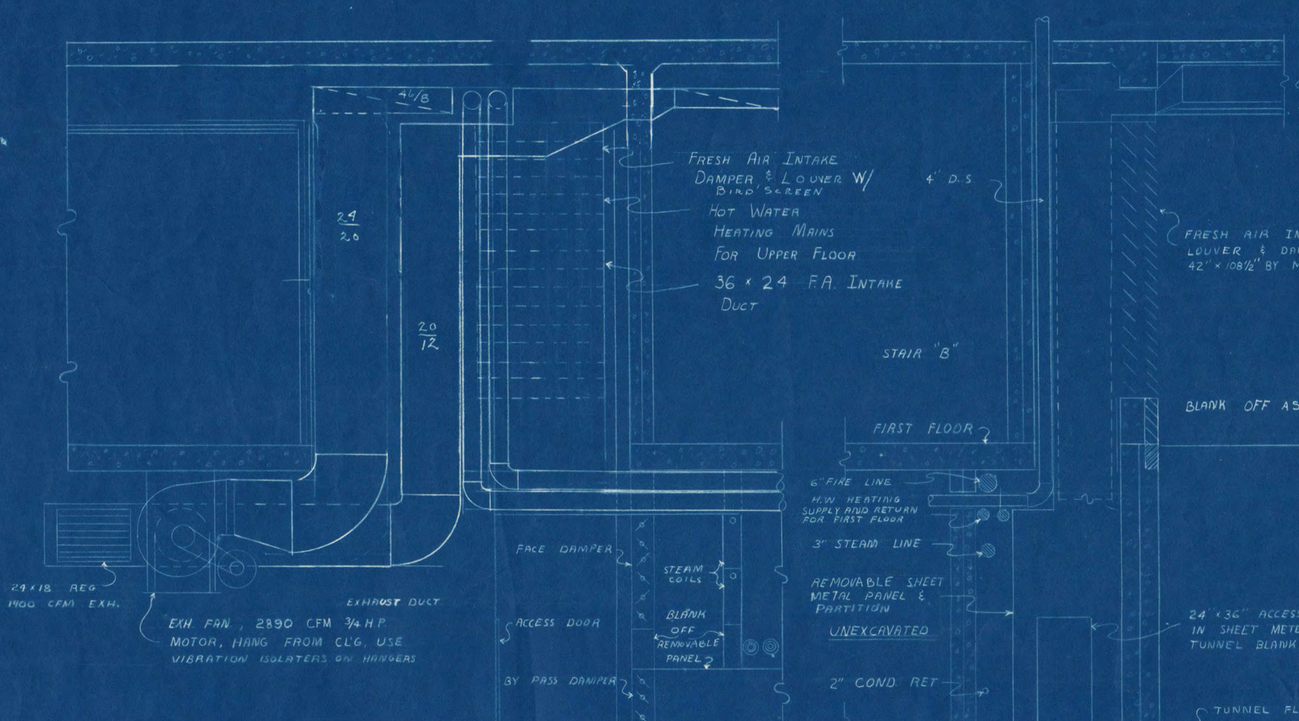
SECTION "B-B" DUCT SHAFT TUNNEL EXHAUST AIR FAN & PREHEAT COILS SCALE 3/8" = 1'-0"
