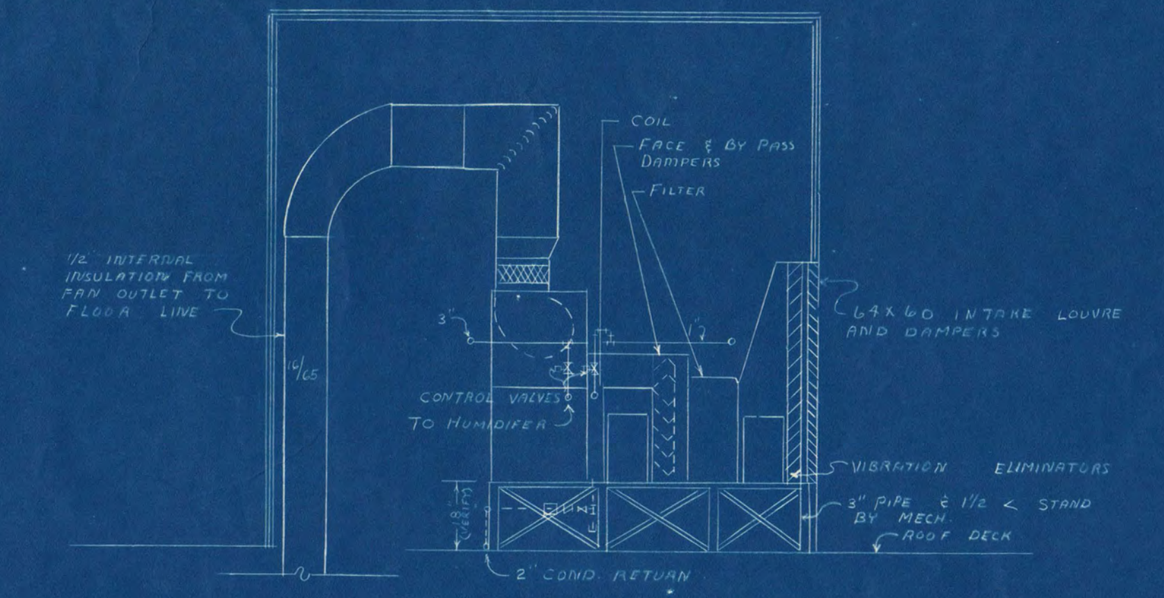
SECTION A-A THRU PENTHOUSE H.V. UNIT SCALE 1/4" = 1'-0"
