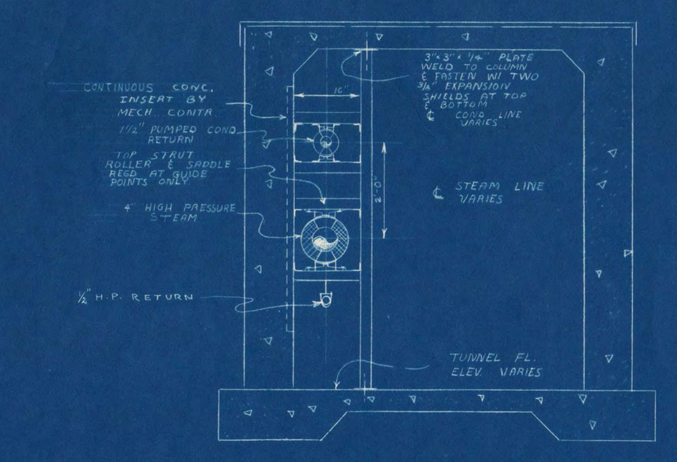
TUNNEL SECTION 2 SCALE 1/2" = 1'-0"
