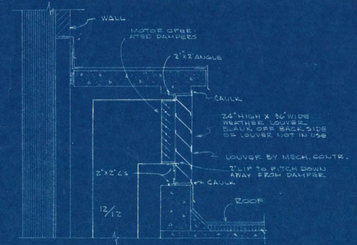
SECTION THROUGH DOGHOUSE SCALE 3/8" = 1'-0"
