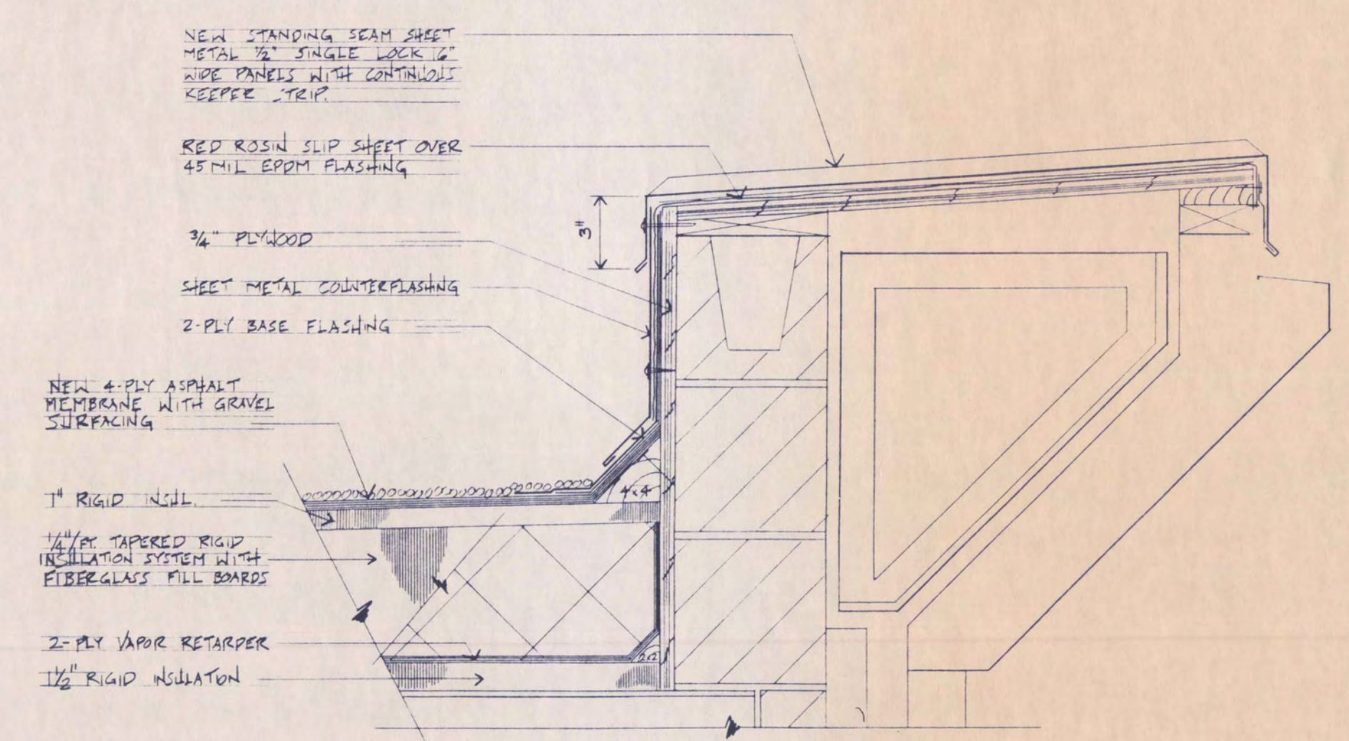
ROOF EDGE DETAIL SCALE 1/8" = 1'-0" (APPROX)
