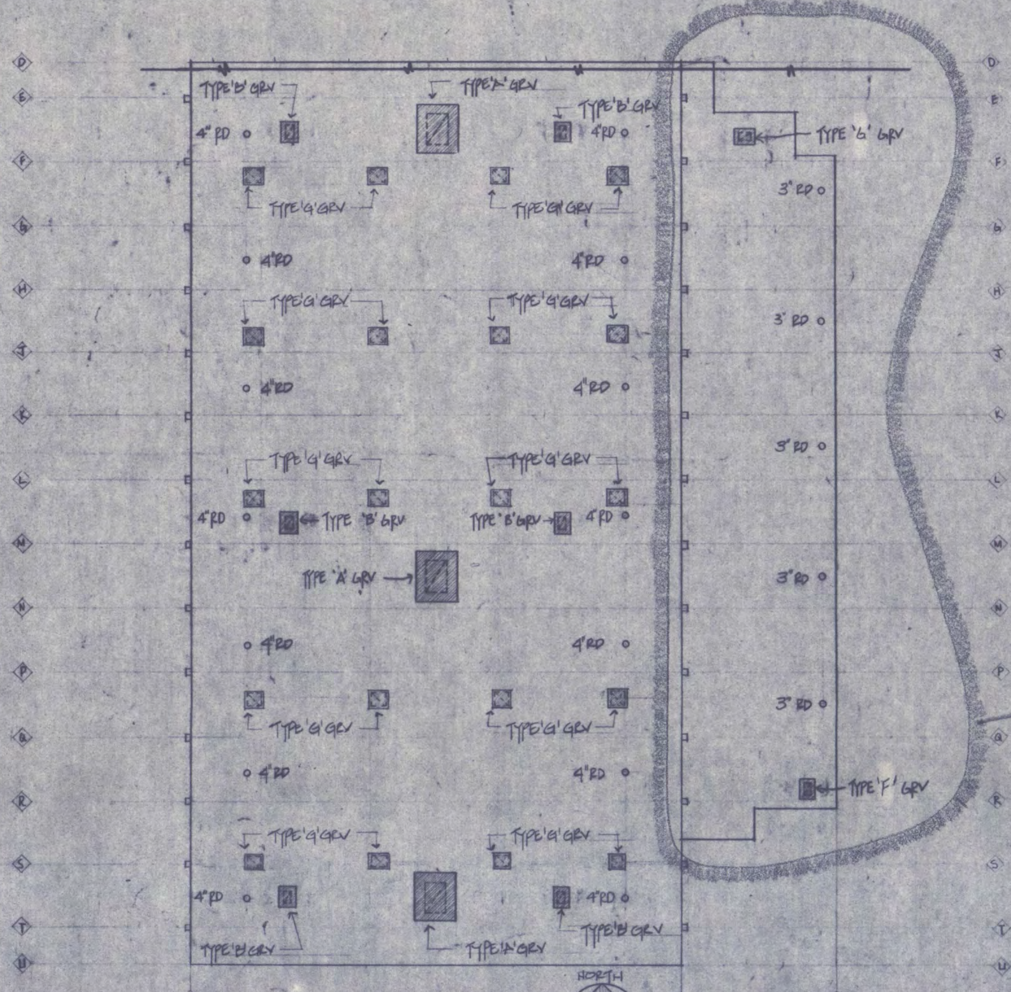
2 ROOF PLAN SCALE: 1/32" = 1'-0"
