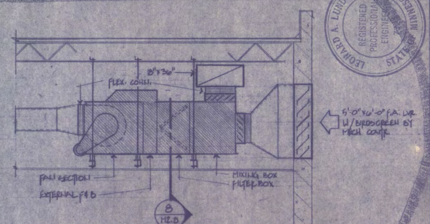
9 WRESTLING ROOM UNIT-ELEVATION SCALE: 1/4" = 1'-0"
