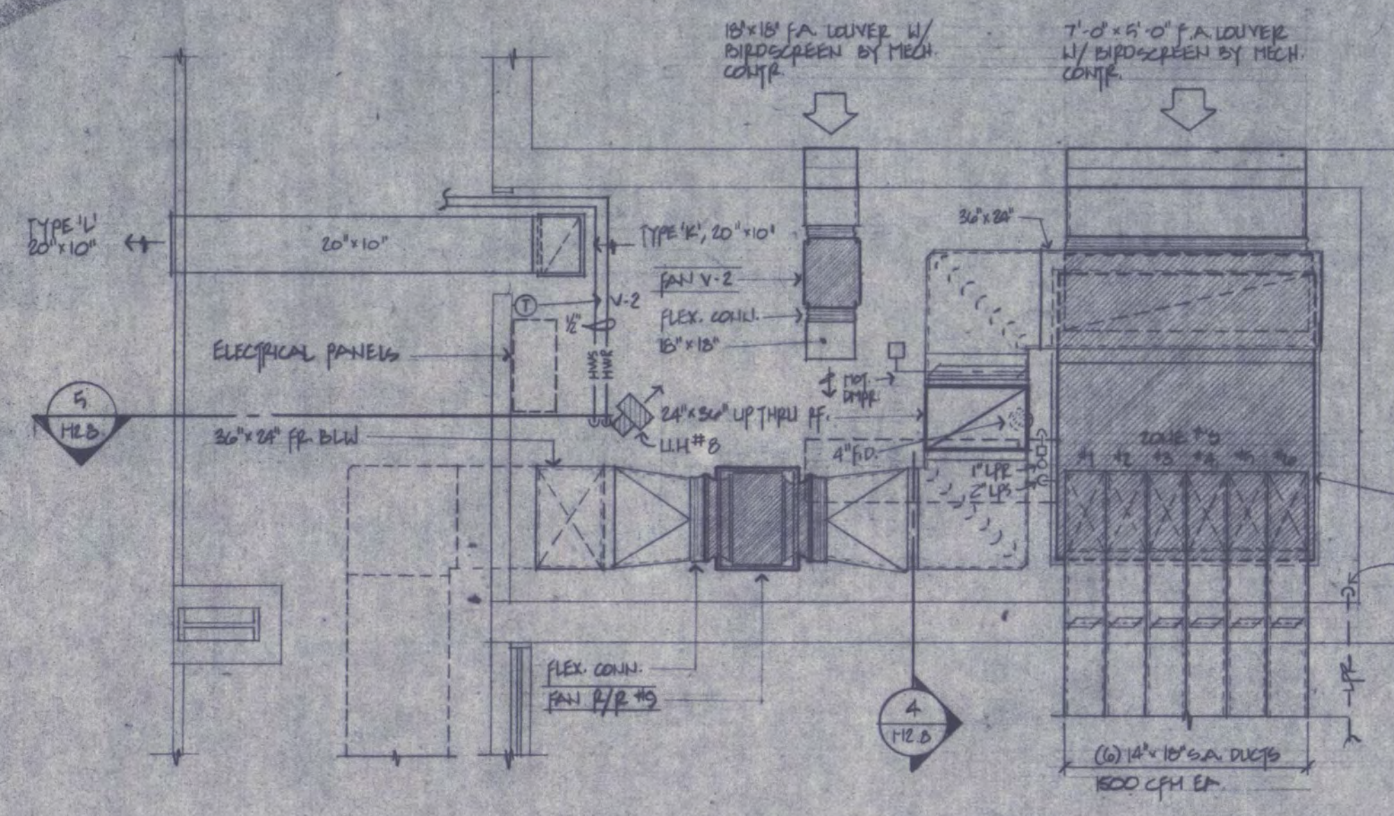
1 MECHANICAL ROOM 225-PLAN (BASE BID) SCALE: 1/4" = 1'-0"
