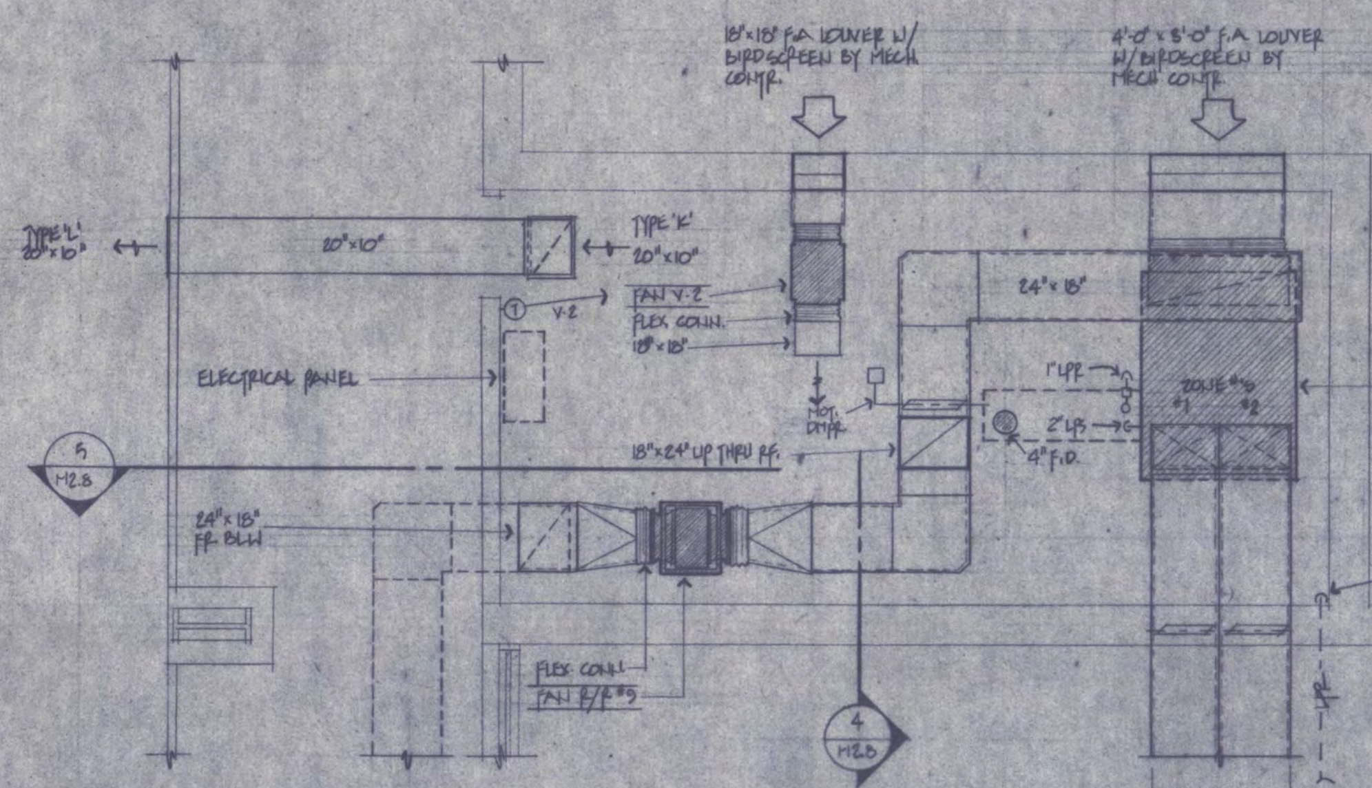
3 MECHANICAL ROOM 225-PLAN (DED. ALT #4) SCALE: 1/4" = 1'-0"
